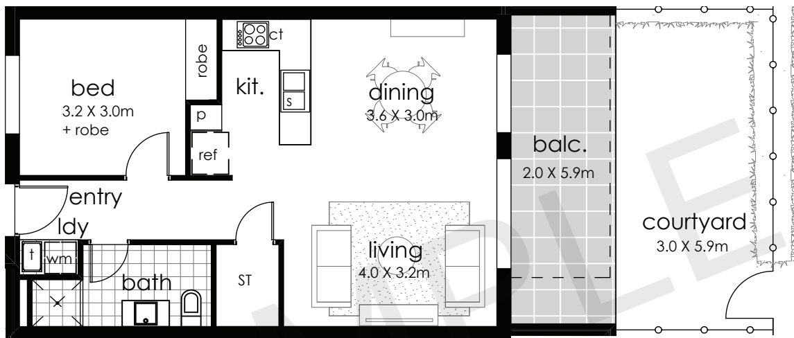
GROUND FLOOR LEVEL PLAN
